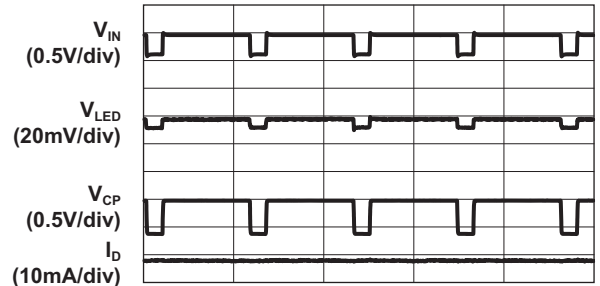
Line Response (1X Mode, 4x30mA Load)
