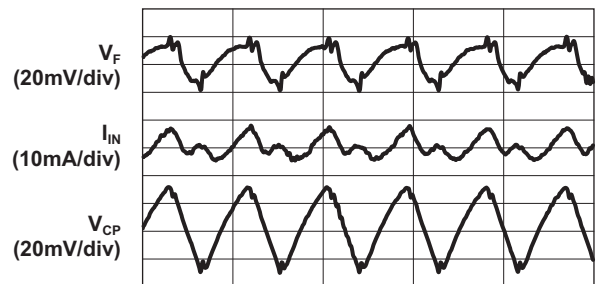
Load Characteristics (1.5X Mode, 4x30mA Load)
